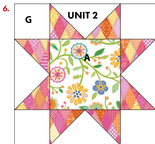
BLOCK 2 make (5)
